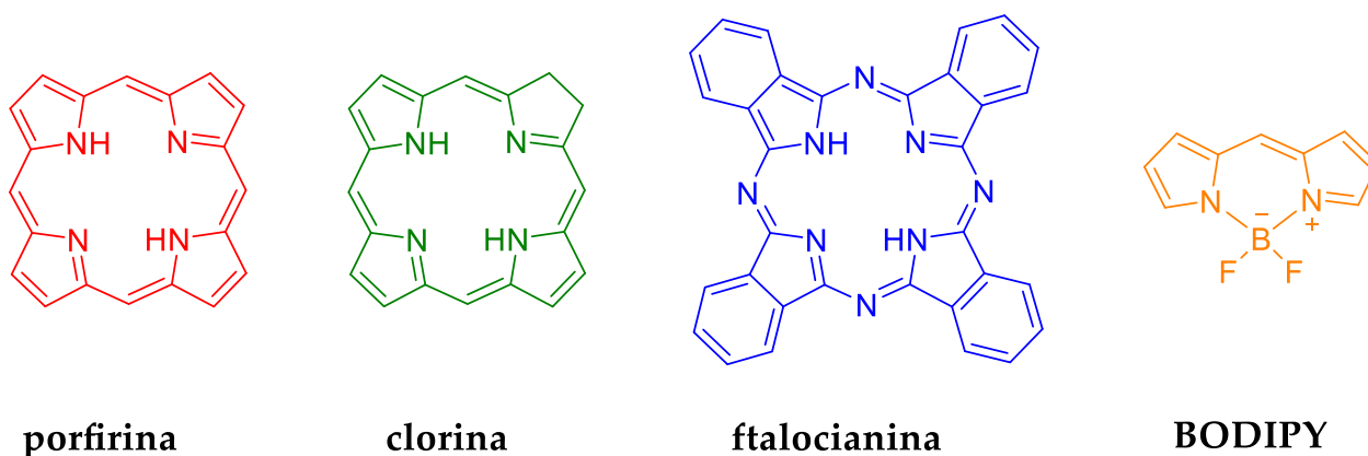
Figura 3. Estructuras generales de las porfirinas, clorinas, ftalocianinas, y BODIPI. Figure 3. General structures of porphyrins, chlorins, phthalocyanines, and BODIPI.
