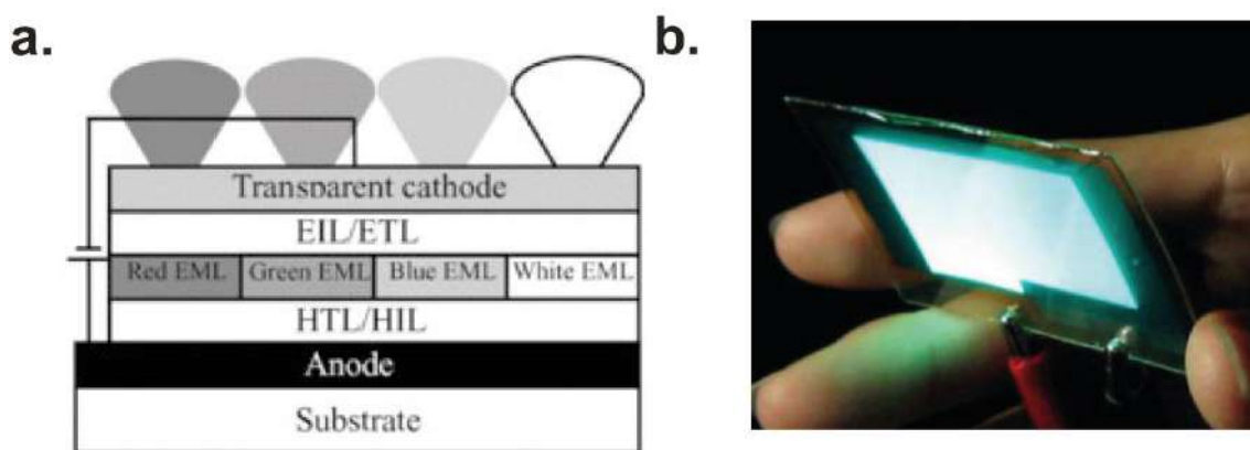
Figure 2. a. Architecture of OLED: hole injection layer (HIL), hole transporting layer (HTL), electron blocking layer (EBL), emitting layer (EML), hole blocking layer (HBL), electron transporting layer (ETL), and electron injection layer (EIL) (Copyright 2010, Wiley), (Chen et al. , 2010); b. Flexible OLED display supported by a transparent cellulose nanofibrils composite film (Copyright 2008, Wiley) (Nogi and Yano, 2008).
