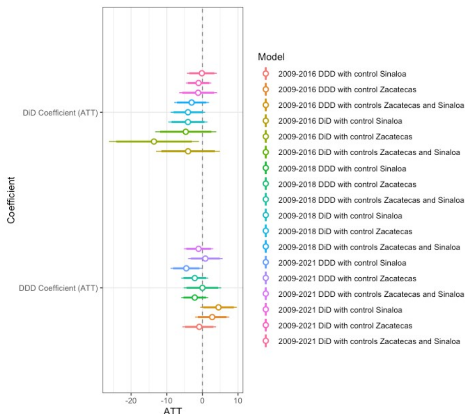
Figure 2. DiD and DDD coefficients of all estimated model specifications.
