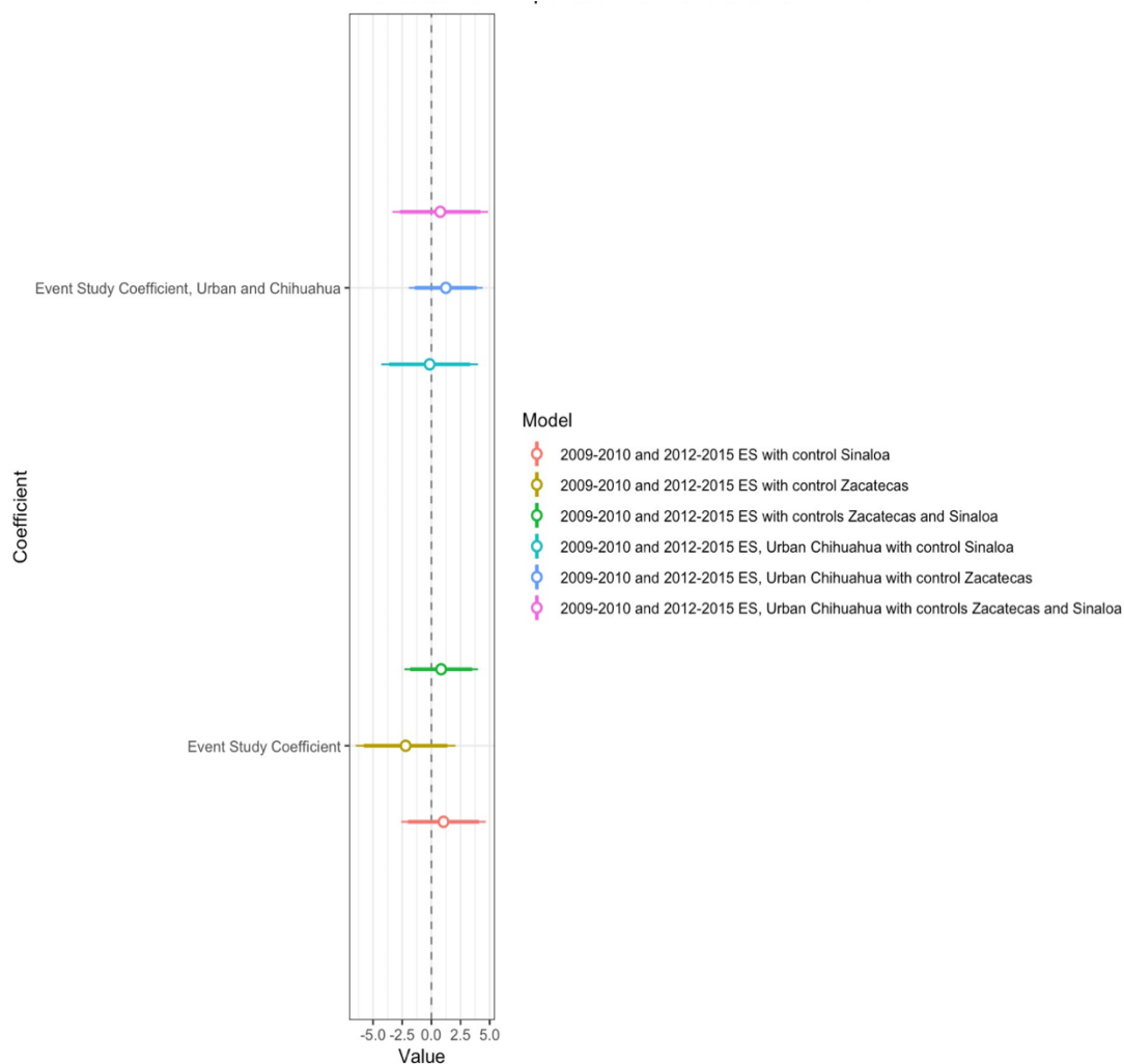
Figure 1. Event studies with periods 2009-2010 and 2012-2015.
